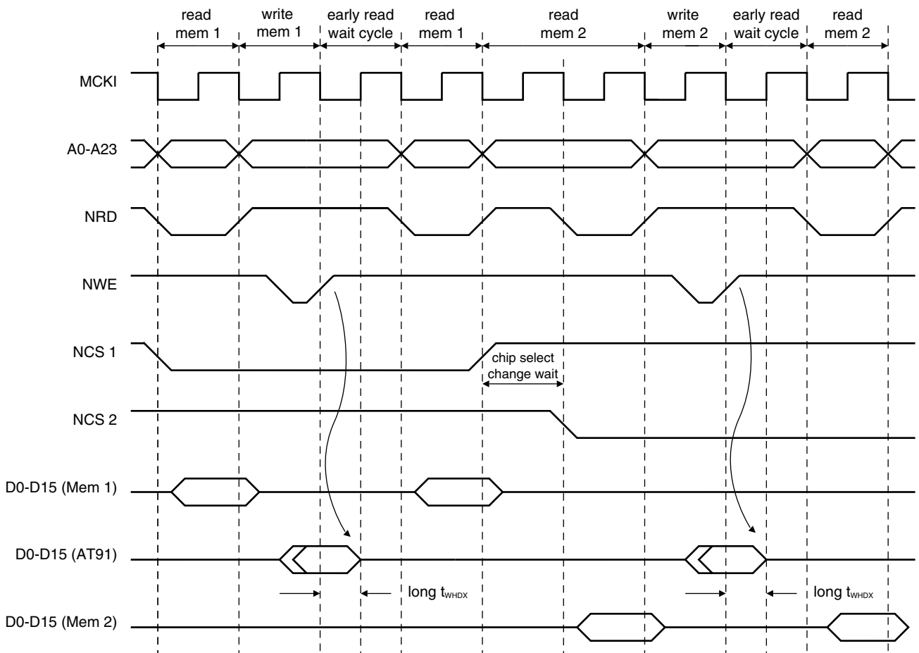
Figure 22. Early Read Protocol with No t_{DP}
